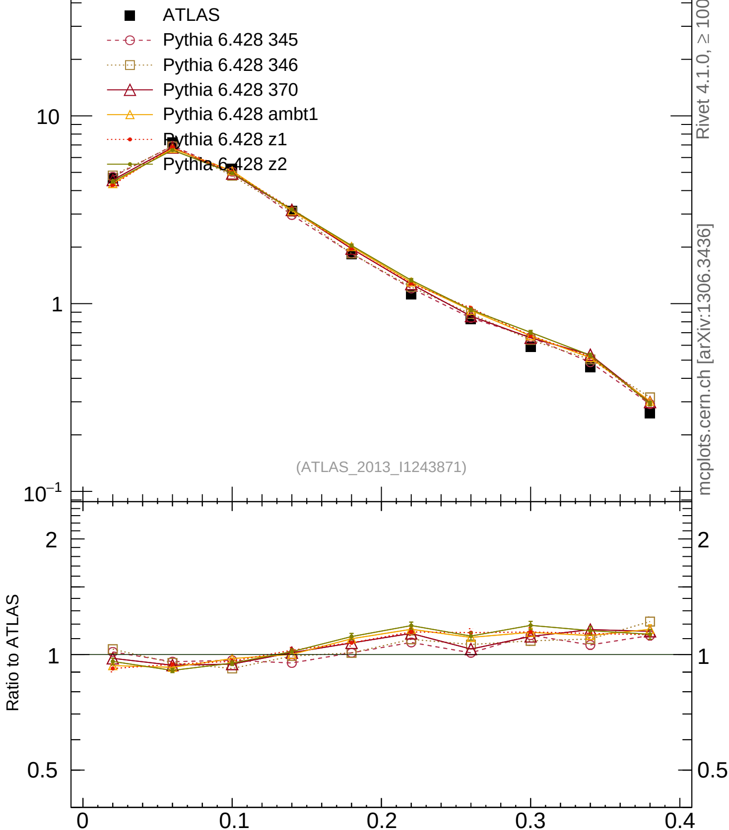
Differential jet shape p (b-jets, p_T > 40 , |\eta| < 2.5 )
